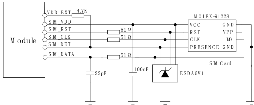
Figure 30: Reference circuit of the 8-pin SIM card holder
